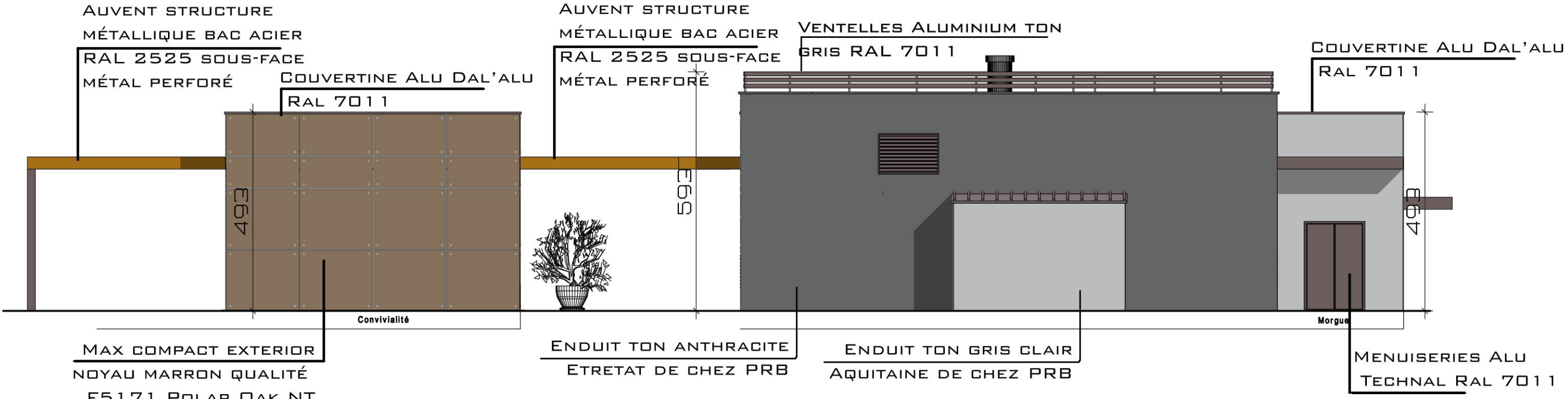
FAÇADE FOUR / TECHNIAUE (NORD)
